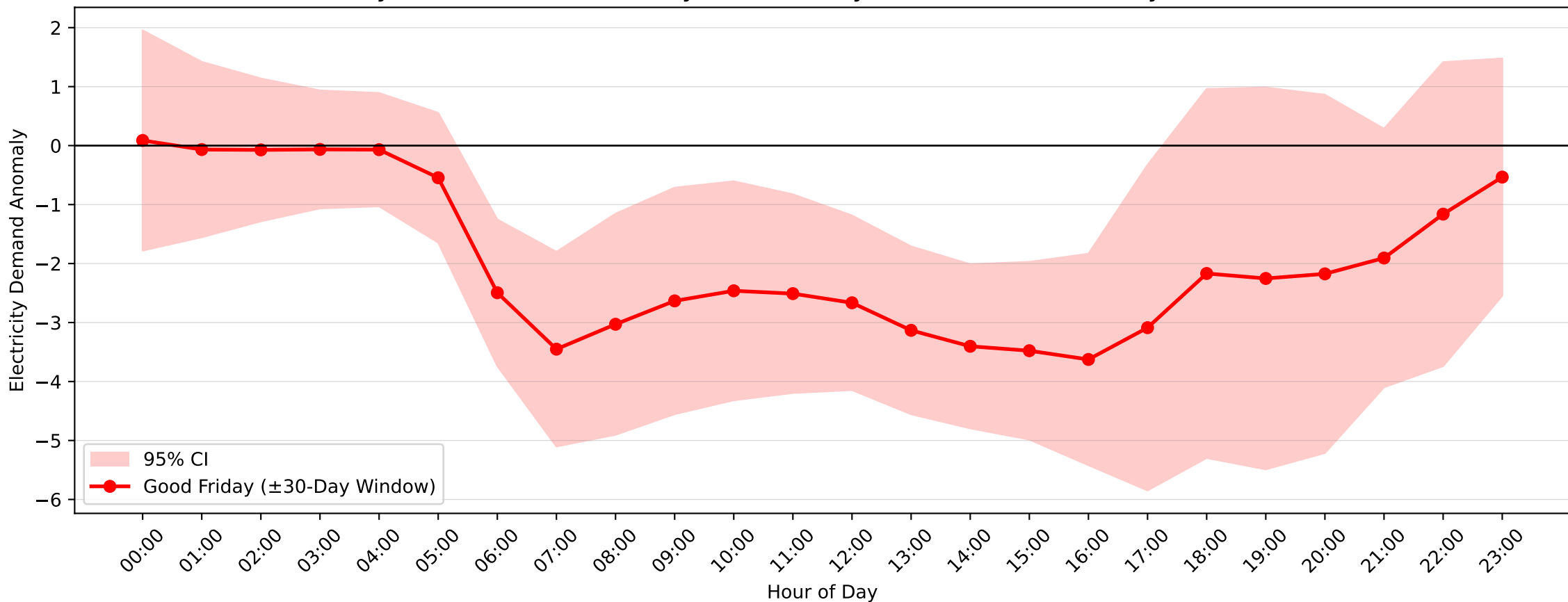
Pymble Demand Anomaly: Good Friday (2004–2017, \pm 30 -Day Window)
